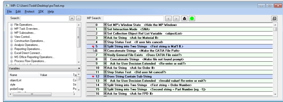
Figure 30-15. Steps 5 and 12 have been set as breakpoints.
